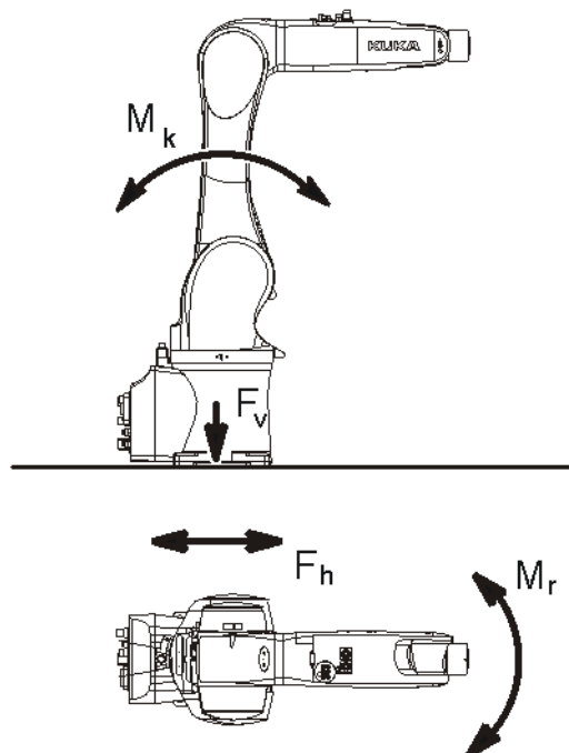
Fig. 4-14: Loads acting on the foundation
