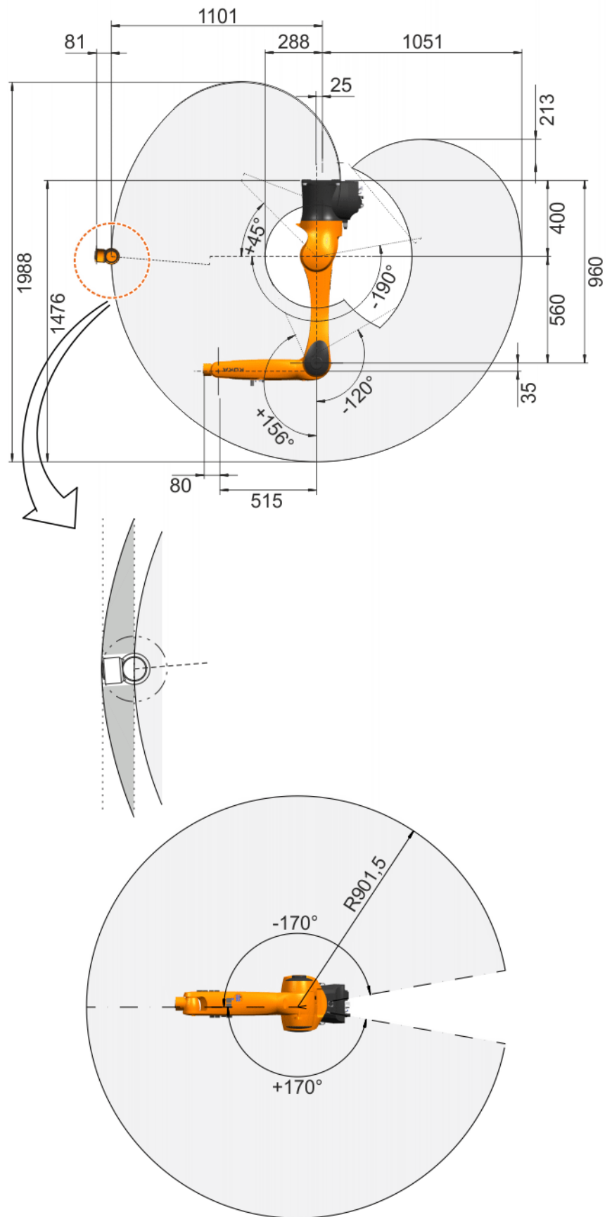
Fig. 4-21: Working envelope, KR 10 R1100 sixx C
