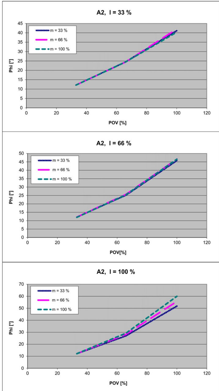
Fig. 4-34: Stopping distances for STOP 1, axis 2
