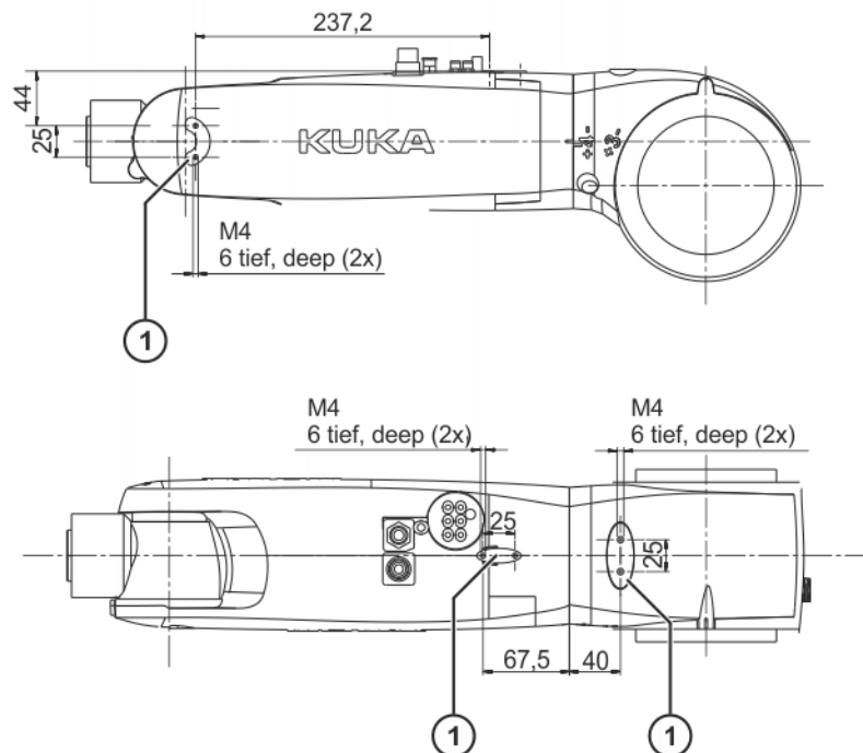
Fig. 4-12: Supplementary load on arm and in-line wrist
