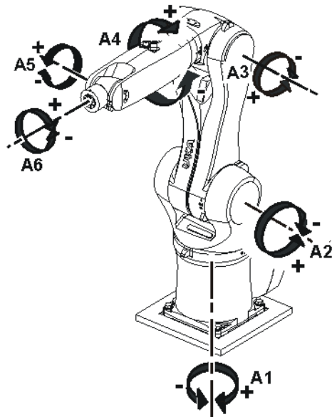
Fig. 4-15: Direction of rotation of robot axes
