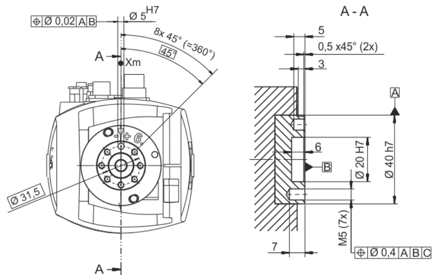
Fig. 4-24: Mounting flange
