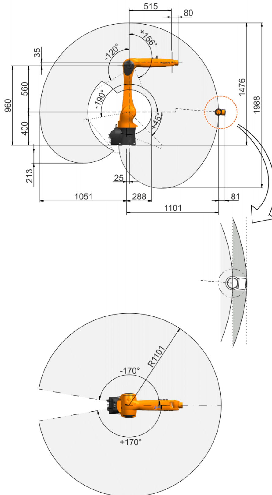
Fig. 4-19: Working envelope, KR 10 R1100 sixx
