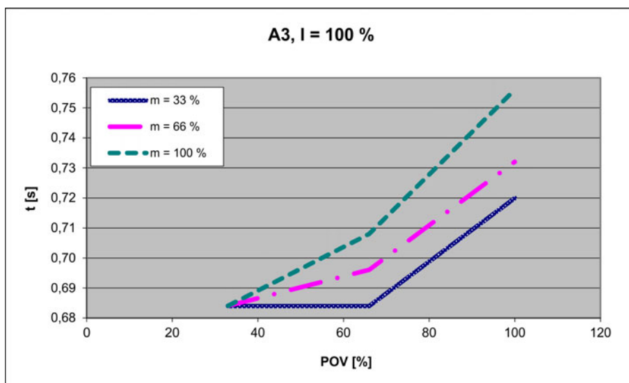
Fig. 4-43: Stopping times for STOP 1, axis 1
