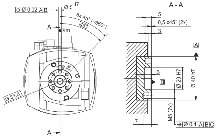
Fig. 4-9: Mounting flange
