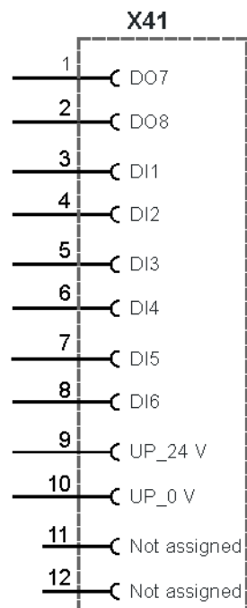
Fig. 6-11: Wiring diagram, connection X41
