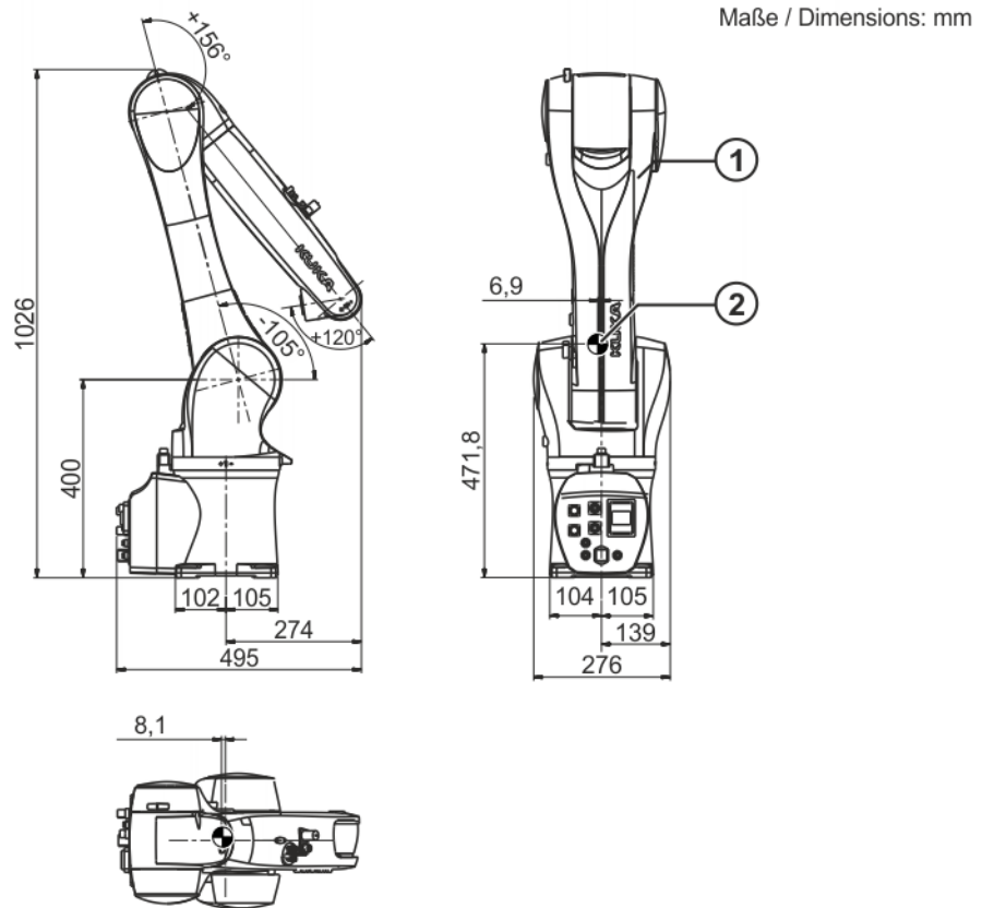
Fig. 7-4: Transport dimensions
