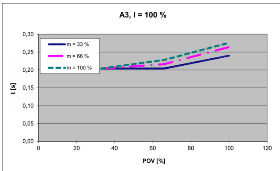
Fig. 4-55: Stopping times for STOP 1, axis 3
