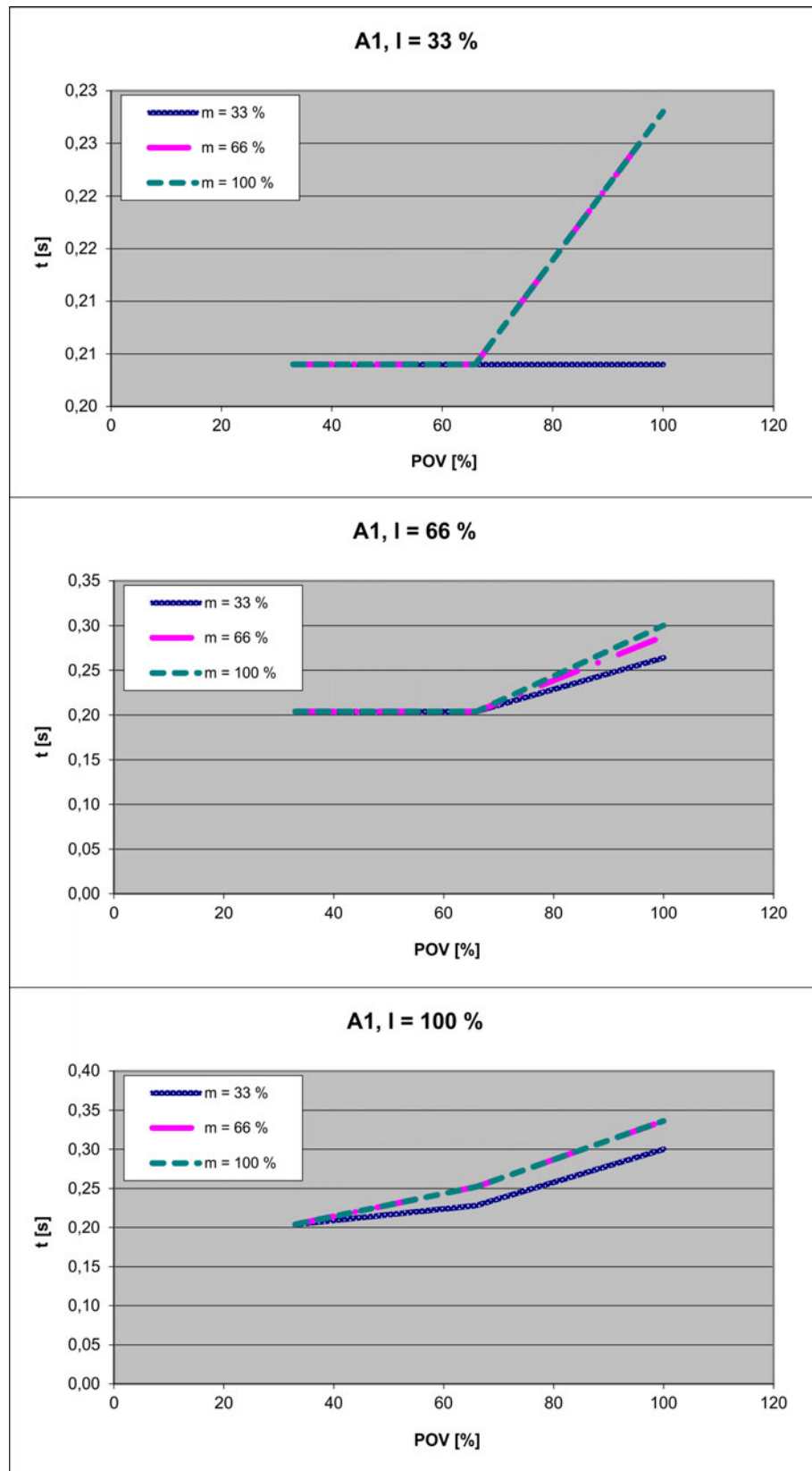
Fig. 4-57: Stopping times for STOP 1, axis 1
