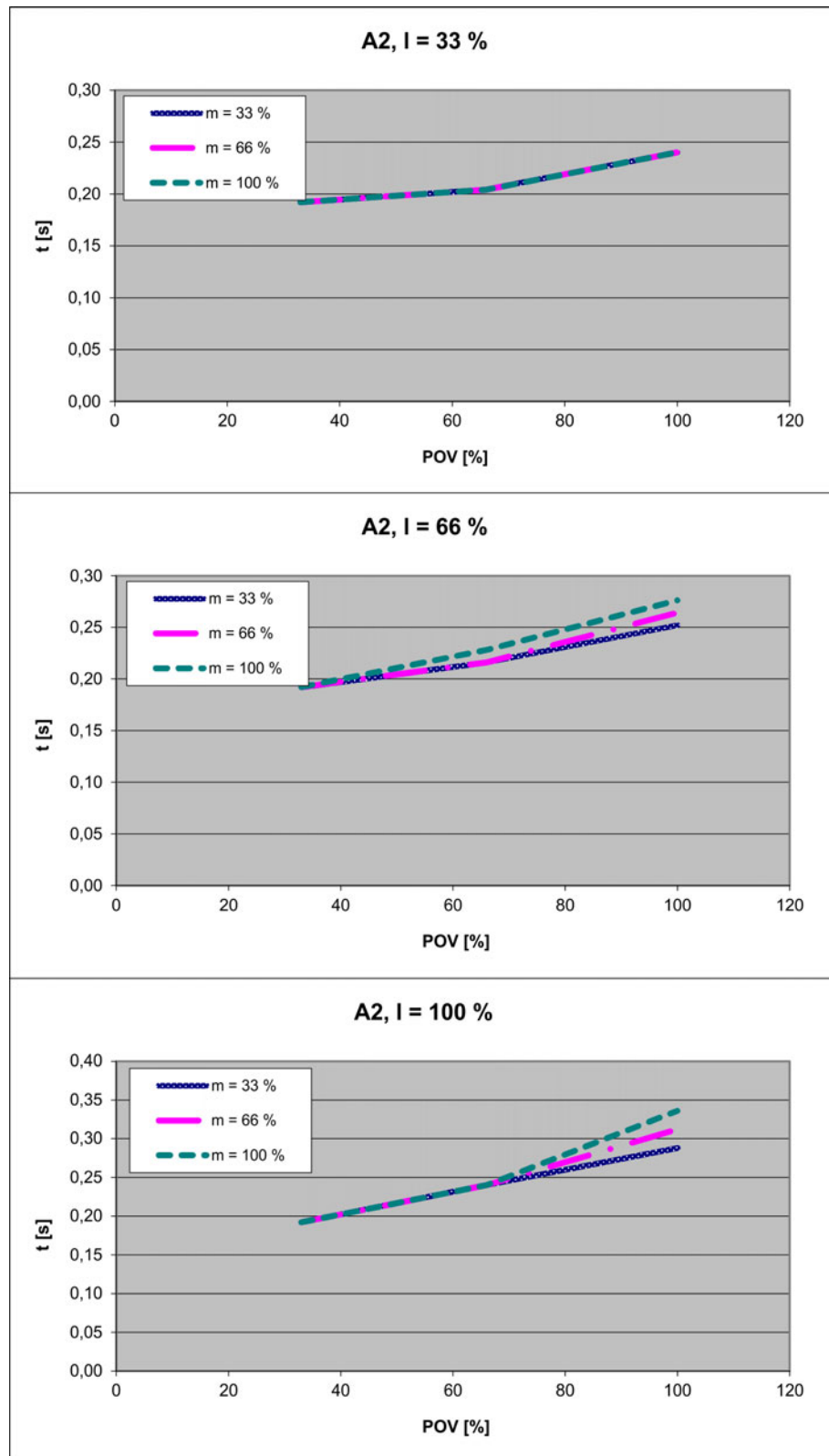
Fig. 4-35: Stopping times for STOP 1, axis 2
