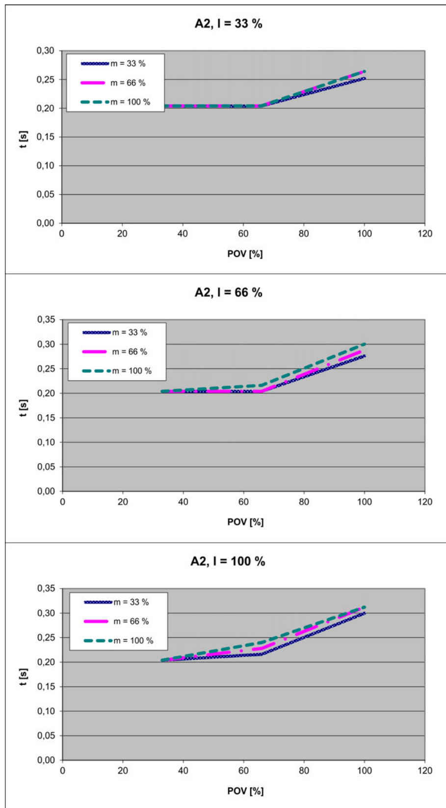
Fig. 4-59: Stopping times for STOP 1, axis 2
