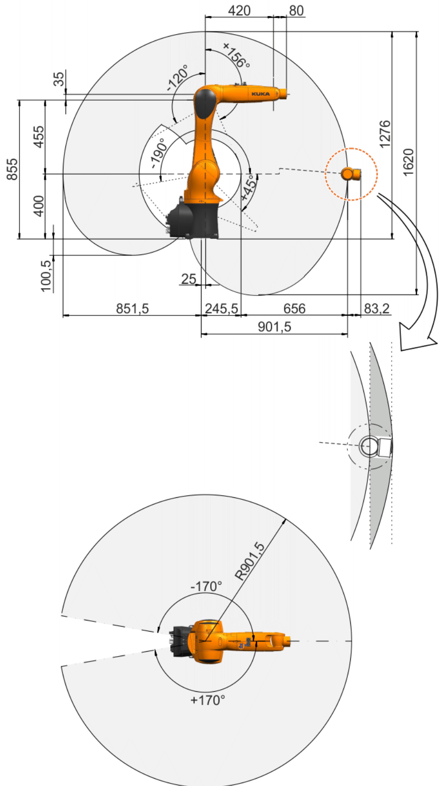
Fig. 4-16: Working envelope, KR 10 R900 sixx
