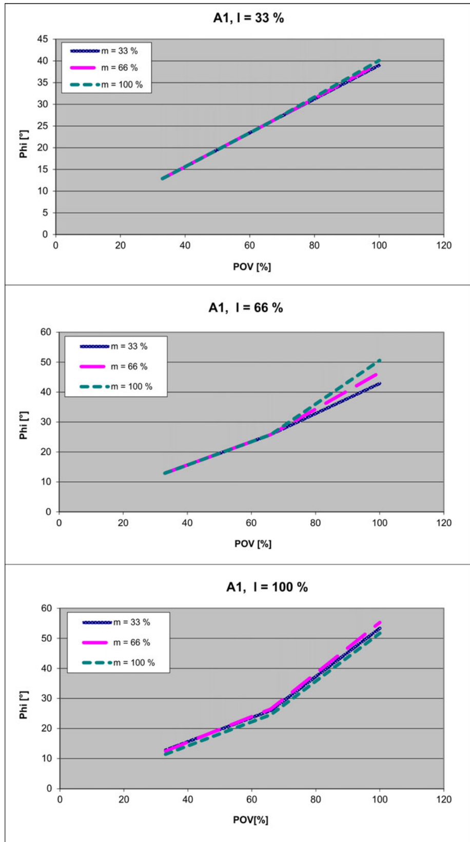
Fig. 4-56: Stopping distances for STOP 1, axis 1
