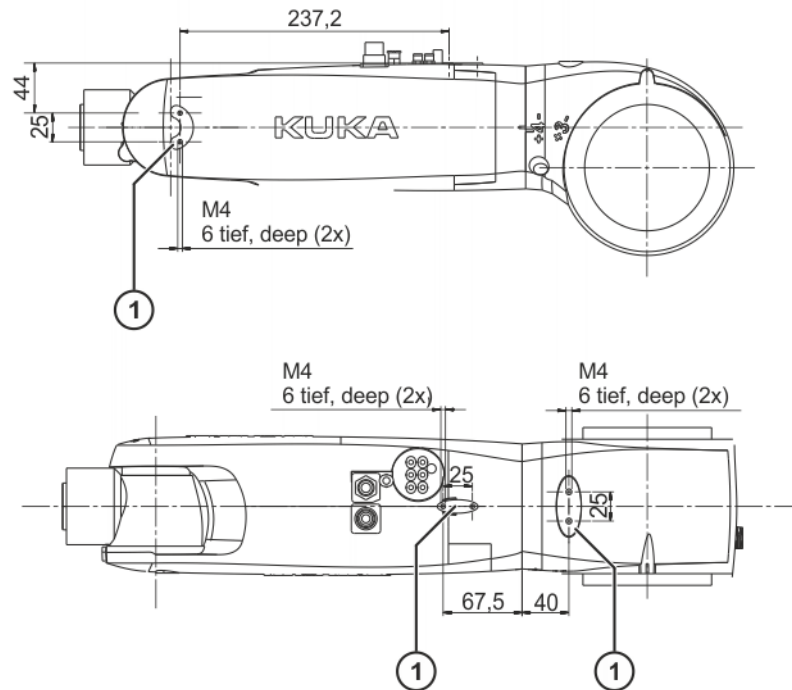
Fig. 4-25: Supplementary load on arm and in-line wrist
