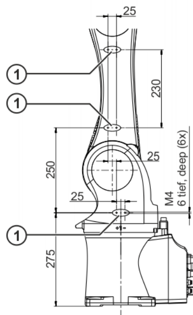
Fig. 4-26: Supplementary load on link arm and rotating column
