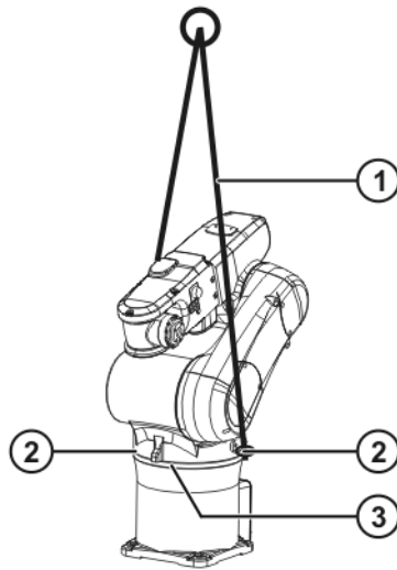
Fig. 5-4: Lifting tackle
