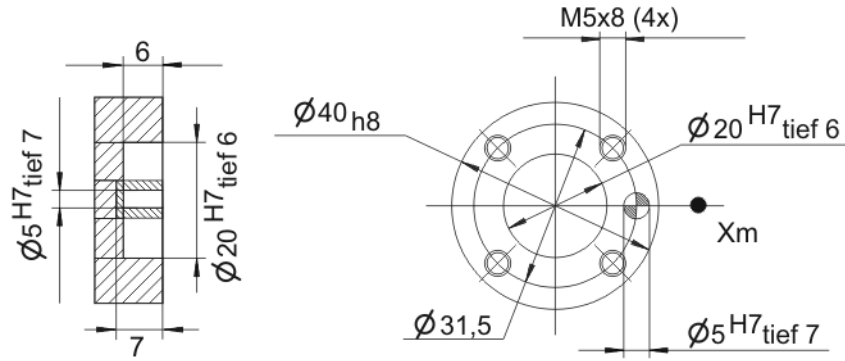
Fig. 2-6: Mounting flange
