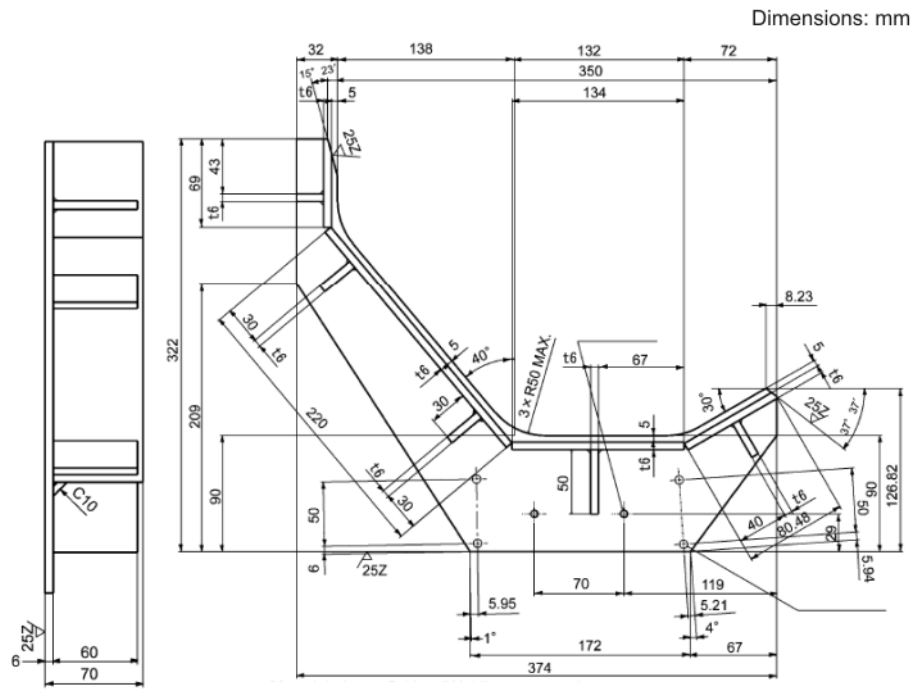
Fig. 6-9: Mechanical stop, dimensioned drawing
