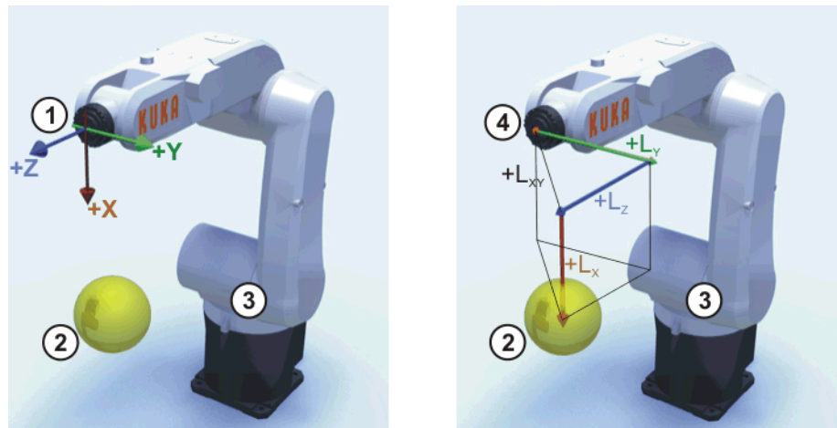
Fig. 2-4: Payload on the robot
