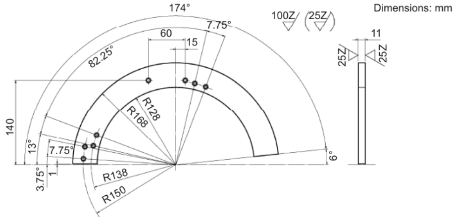
Fig. 6-1: Plate, dimensioned drawing
