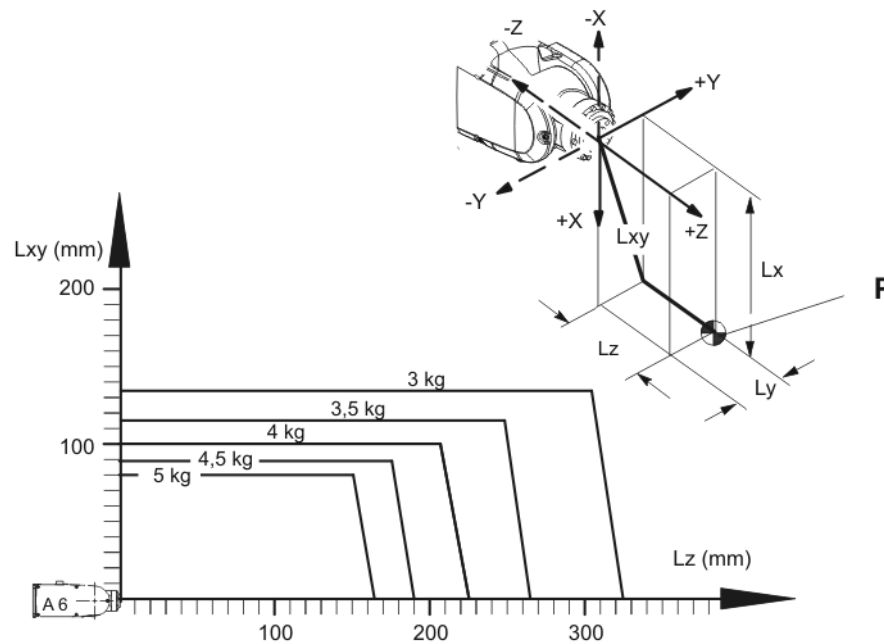
Fig. 2-5: Payload diagram
