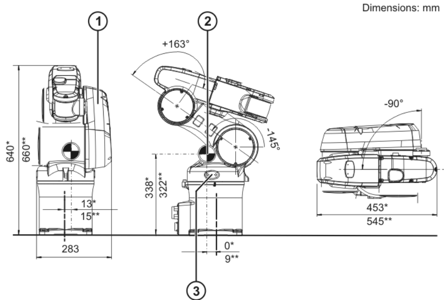
Fig. 5-2: Transport dimensions
