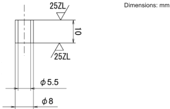
Fig. 6-10: Spacer, dimensioned drawing
