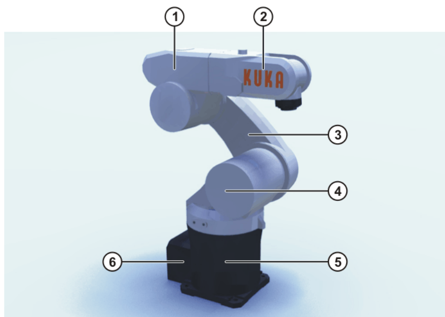
Fig. 1-2: Principal components
