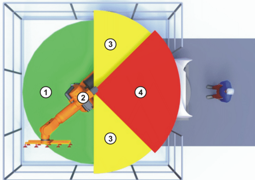
Fig. 3-1: Example of axis range A1
